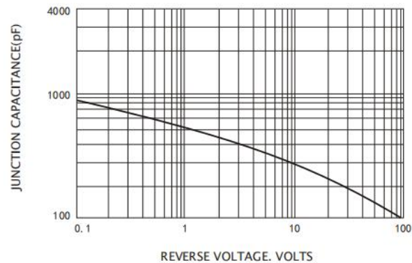
Figure 5: Capacitance Characteristics
