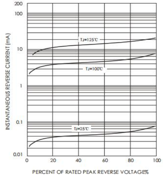
Figure 4: Reverse Characteristics
