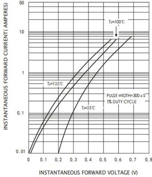
Figure 3: Forward Characteristics
