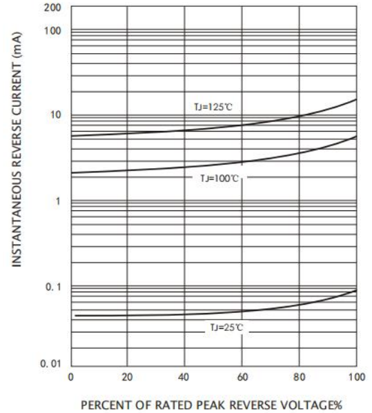
Figure 4: Reverse Characteristics
