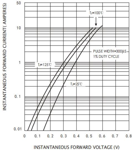
Figure 3: Forward Characteristics
