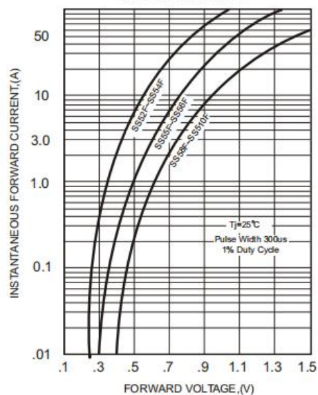
FIG.2-TYPICAL FORWARD CHARACTERISTICS
