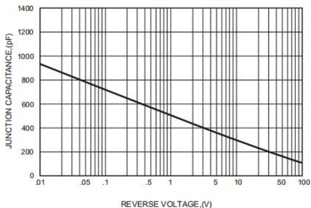
FIG.4-TYPICAL JUNCTION CAPACITANCE
