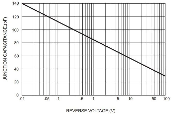
FIG.5-TYPICAL JUNCTION CAPACITANCE
