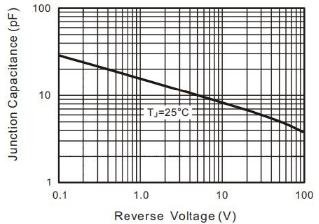
Figure 4: Junction Capacitance
