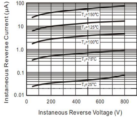
Figure 2: Reverse Characteristics
