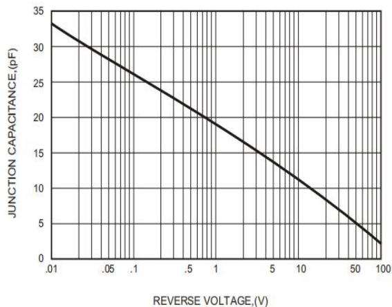
Figure 4: Junction Capacitance
