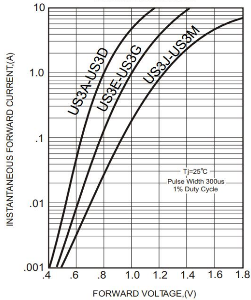
FIG.1-TYPICAL FORWARD CHARACTERISTICS
