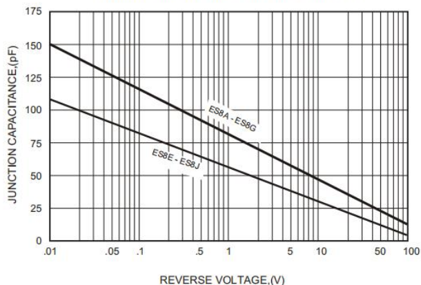
FIG.6-TYPICAL JUNCTION CAPACITANCE
