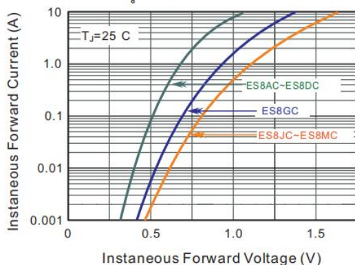
FIG.3-TYPICAL FORWARD CHARACTERISTICS
