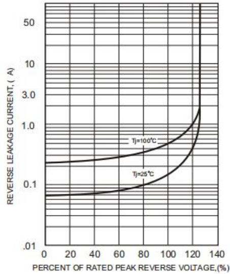
FIG.4-TYPICAL REVERSE CHARACTERISTICS
