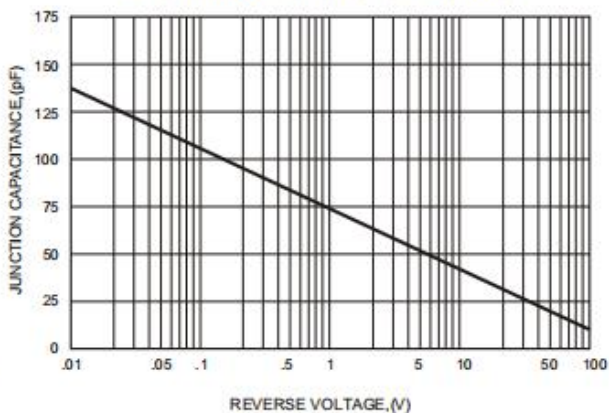
FIG.6-TYPICAL JUNCTION CAPACITANCE
