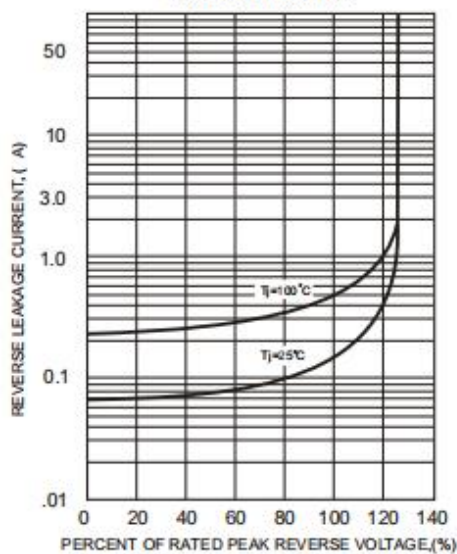
FIG.4-TYPICAL REVERSE CHARACTERISTICS
