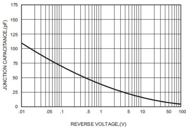
FIG.6-TYPICAL JUNCTION CAPACITANCE
