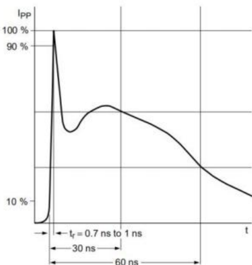
IEC61000-4-2 Waveform
