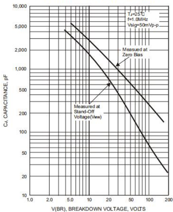
FIG.4-TYPICAL JUNCTION CAPACITANCE
