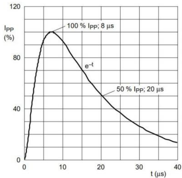
IEC 61000-4-5 Waveform( 8/20 \mu s pulse)
