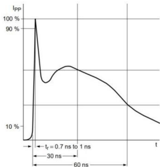
IEC61000-4-2 Waveform
