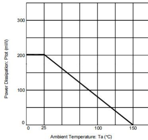
Figure 4: Derating Curve
