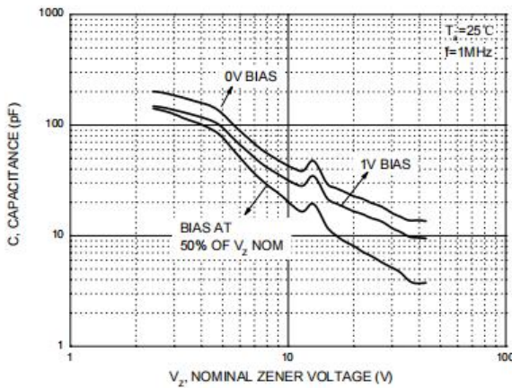
Figure 2: Capacitance Characteristics
