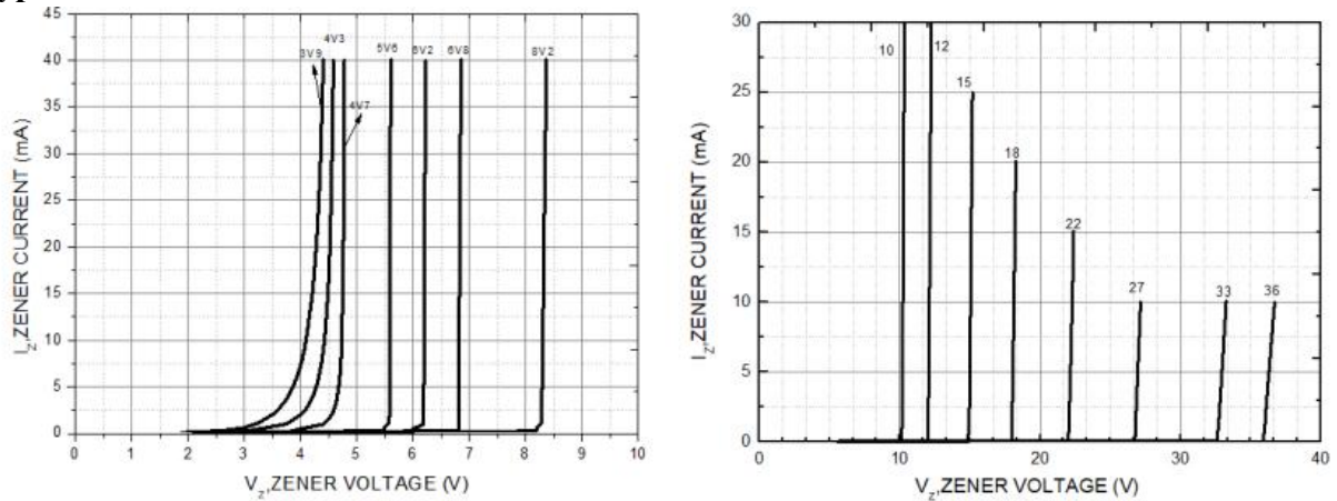
Figure 1: Zener Characteristics
