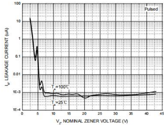
Figure 3: Leakage Current
