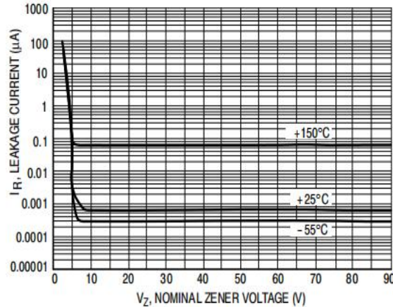
Figure 5: Leakage Current
