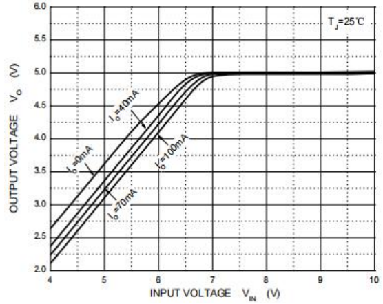
Figure 2: Dropout Characteristics
